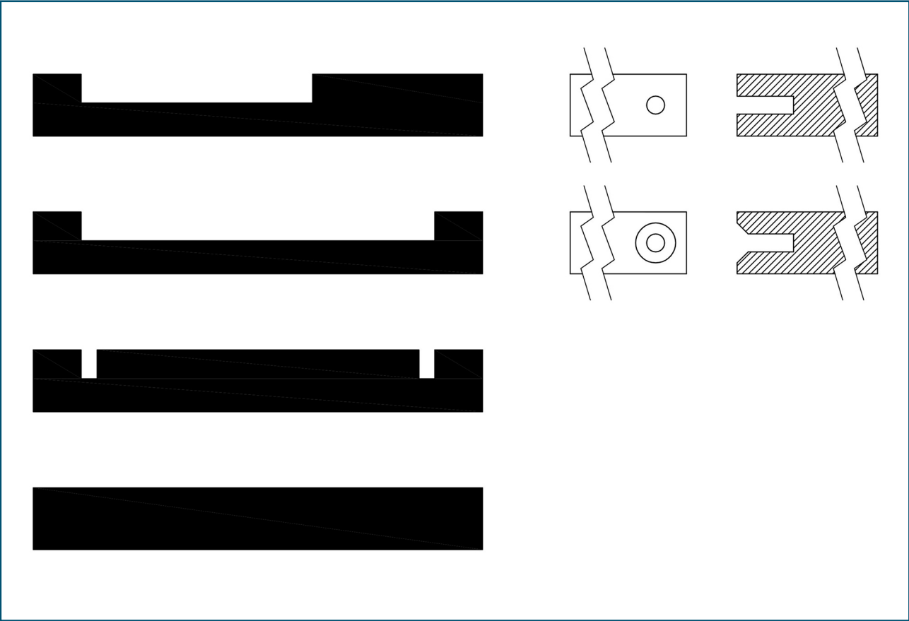
Examples of standard machining. Workmanship at customer's design
